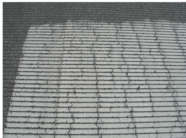
FIGURE 6-12. THE HEAVIER PAINT IN THE OVERLAP AREA CAUSED THE PAINT AND THE ASPHALT TO CRACK.
