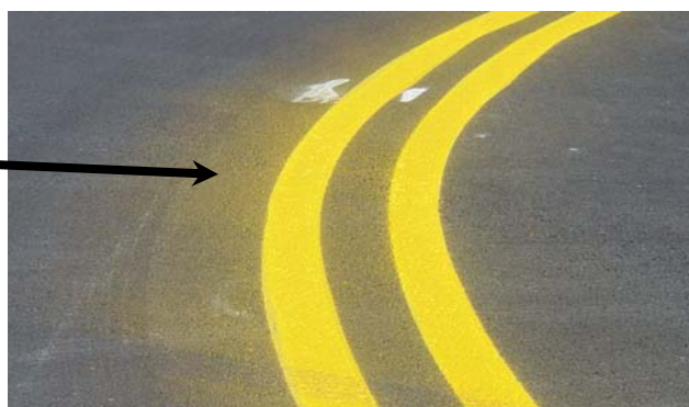
FIGURE 6-45. CLOSE UP OF OVER SPRAY IN FIGURE 6-44.
