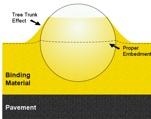
FIGURE 6-65. WICKING MATERIAL OVER BEAD.
