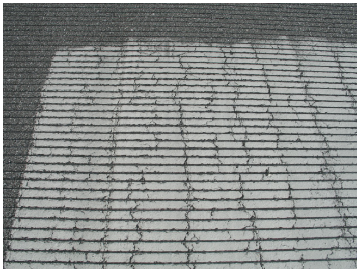
FIGURE 4-12. PAINT BONDS BETTER TO ASPHALT THAN ASPHALT DOES TO ITSELF.
